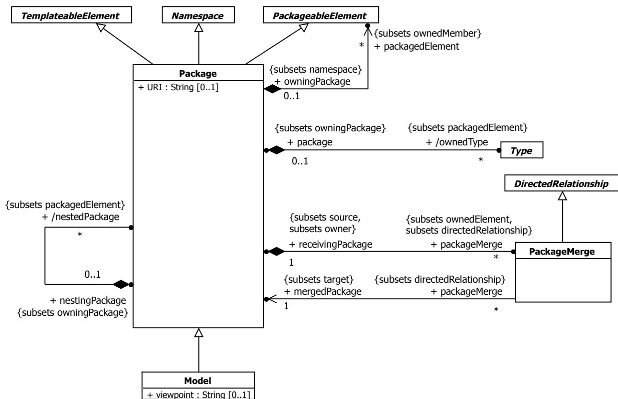
Figure 12.1 Packages
