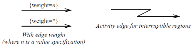
Figure 15.7 ActivityEdge notation
